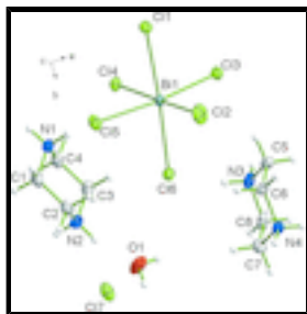
Fig. 1. The asymmetric unit of the title compound with atom labels. Displacement ellipsoids were drawn at the 30% probability level
